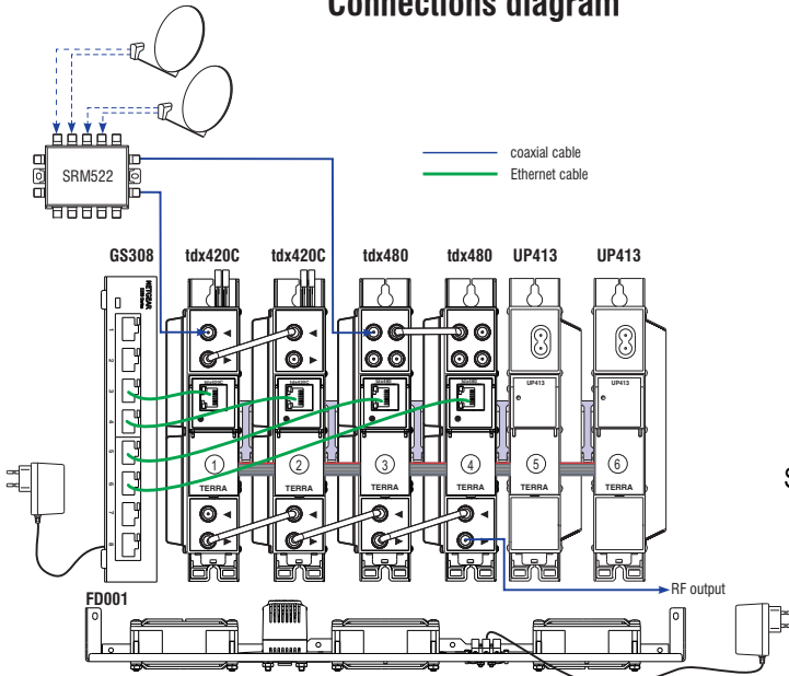
Connections diagram
